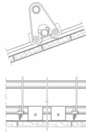
Double pipe system with ice breaker
