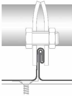
Detail of clamp on standing seam
