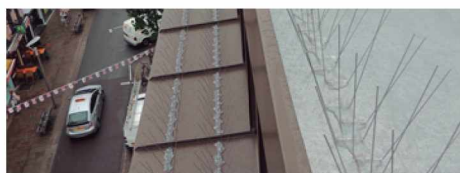
Bird spikes attached using neutral curing silicone
