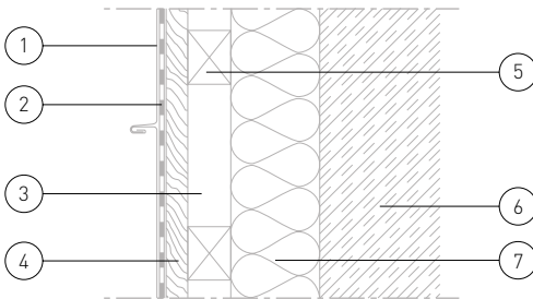
Horizontal section through elZinc® titanium zinc facade with timber substructure
